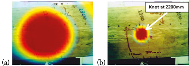
Figure 10: Microphone phased array (a) beamforming and (b) CLEANSC plots imaging the sound coming from the wooden pole in the lab. The plots show peaks in the vicinity of a knot, located 2200 mm from the source.
