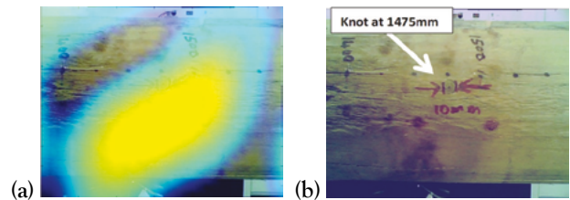
Figure 11: Plots showing an example where the microphone phased array (a) beamforming and (b) CLEANSC plots did not show any peaks in the vicinity of a knot, located at 1475 mm for the wooden pole in the lab
