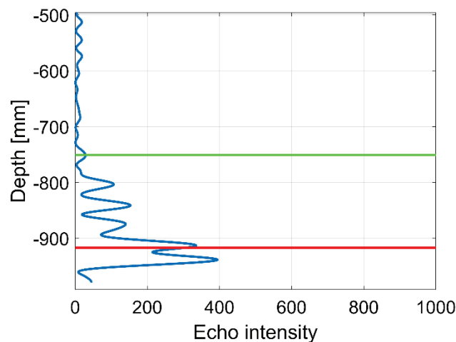
Figure 4. An ultrasonic profile of pasture after matched filtering (blue). Also shown are the top of the pasture (green) and the ground position (red) measured manually with a tape.
