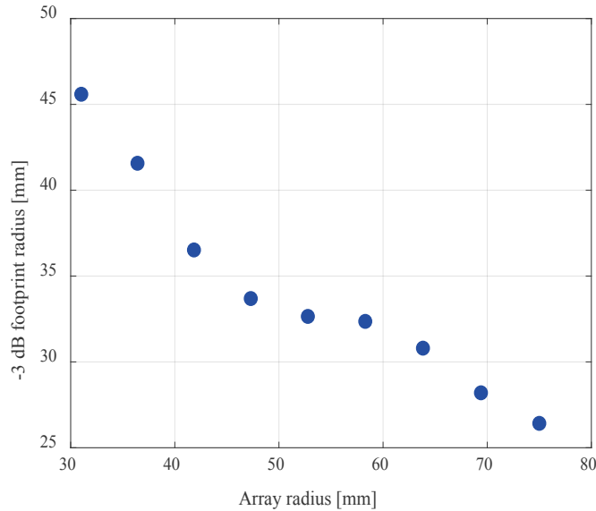
Figure 2. The half-power footprint radius at a range of 850 mm for a 20-35 kHz linear FM chirp and matched filter.
