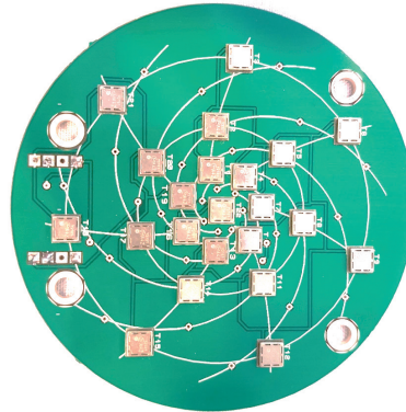
Figure 1. The basic spiral array with transmitting elements shown, and microphones sensing through the small apertures on the marked spirals.
