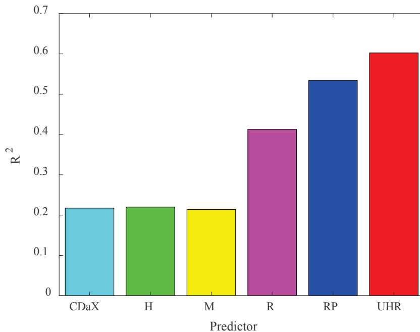
Figure 5. Coefficient of determination, R^2 , between direct biomass measurement and predictor variables CDaX pasture depth (cyan), ultrasonic pasture depth (green), manual tape measurement (yellow), ultrasonic reflectivity (magenta), rising plate clicks (blue), and combined ultrasonic depth and reflectivity (red).
