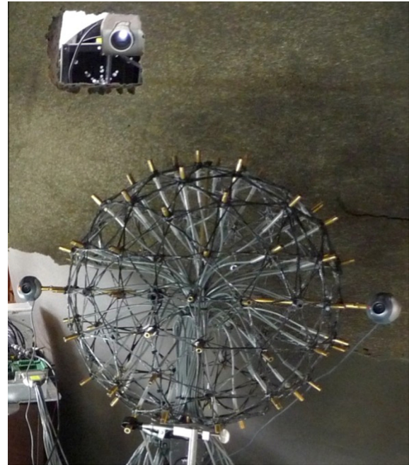
Fig. 2. Structured light experimental setup for a spherical microphone array containing three cameras and a data projector used to obtain 3D surface scans of an object for acoustic imaging.
