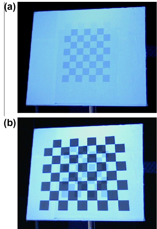
Fig. 3. Calibration rig used for structured light calibration. Image (a) shows the printed checkerboard pattern, which is glued onto its surface. A second checkerboard pattern, which is projected onto the calibration rig, is shown in image (b).
